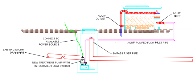
Aquip 10 integrated to a catch basin
