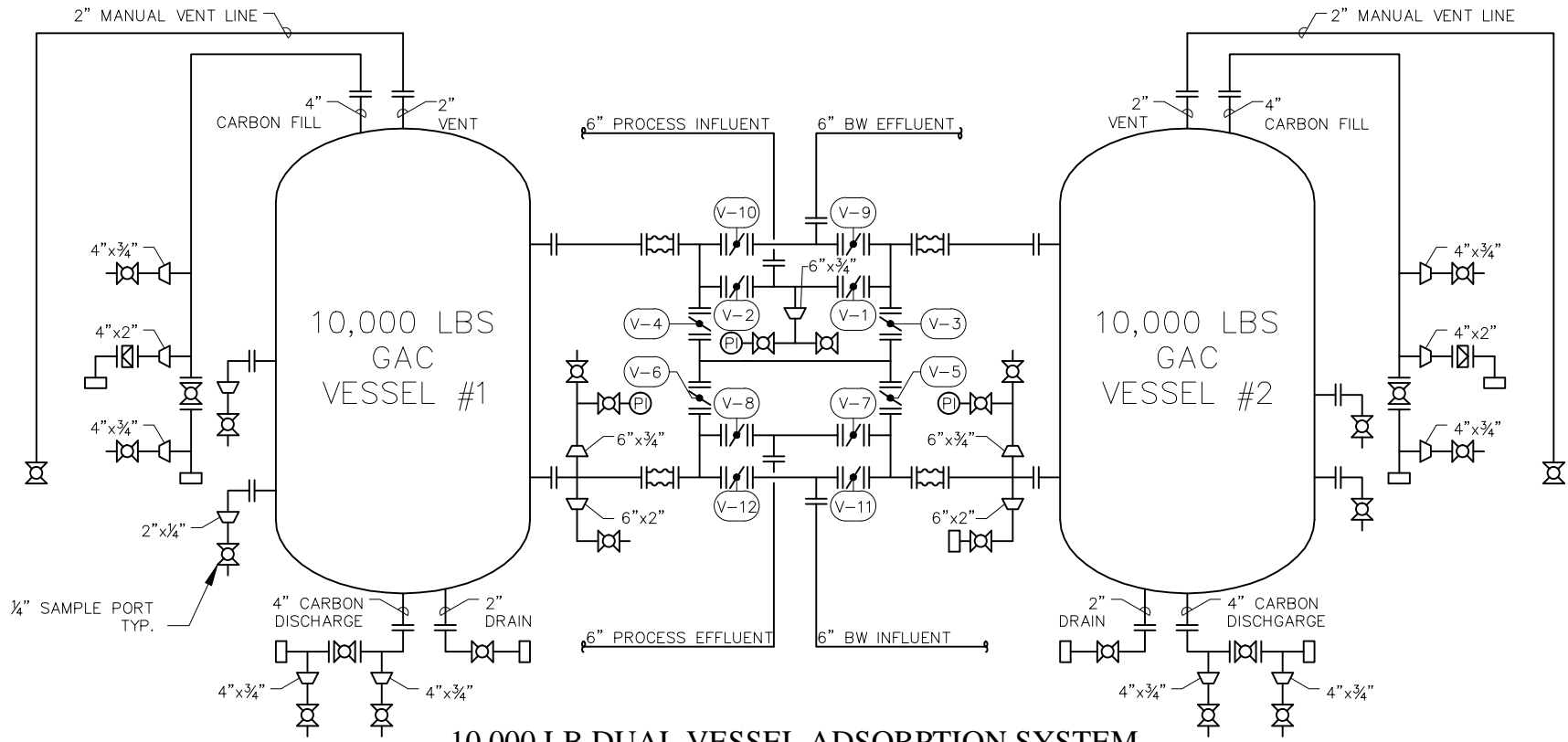
10,000 LB DUAL VESSEL ADSORPTION SYSTEM
